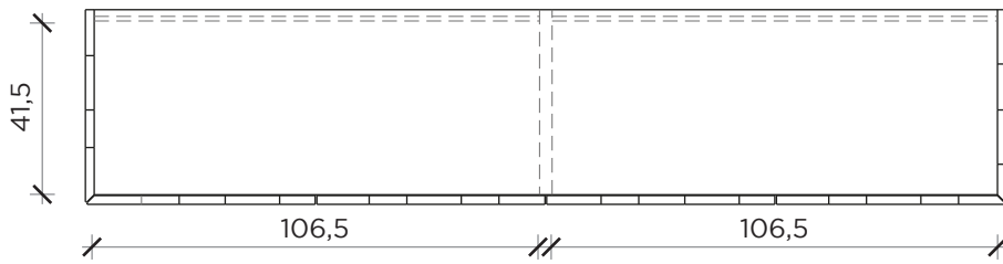
FRONTE | FRONT
