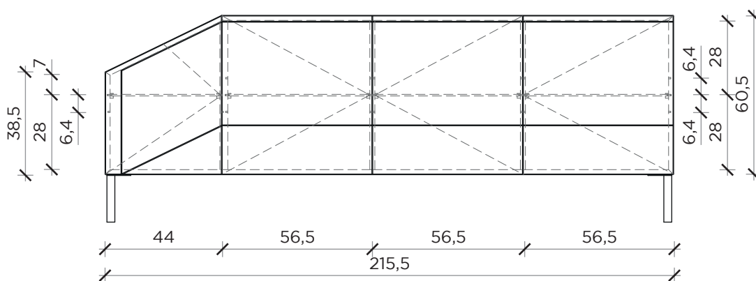
FRONTE | FRONT
