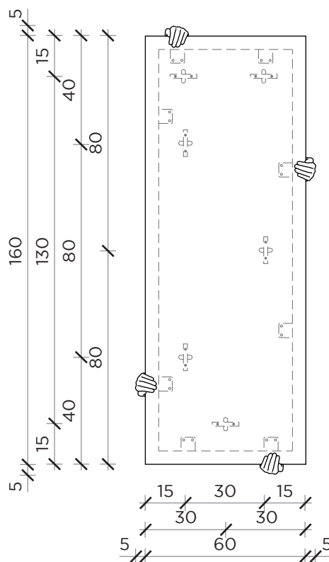
FRONTE | FRONT
