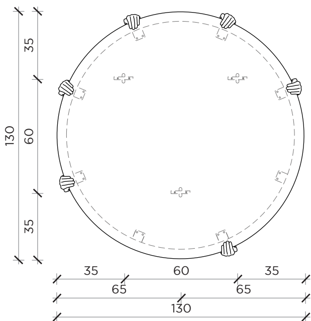
FRONTE | FRONT
