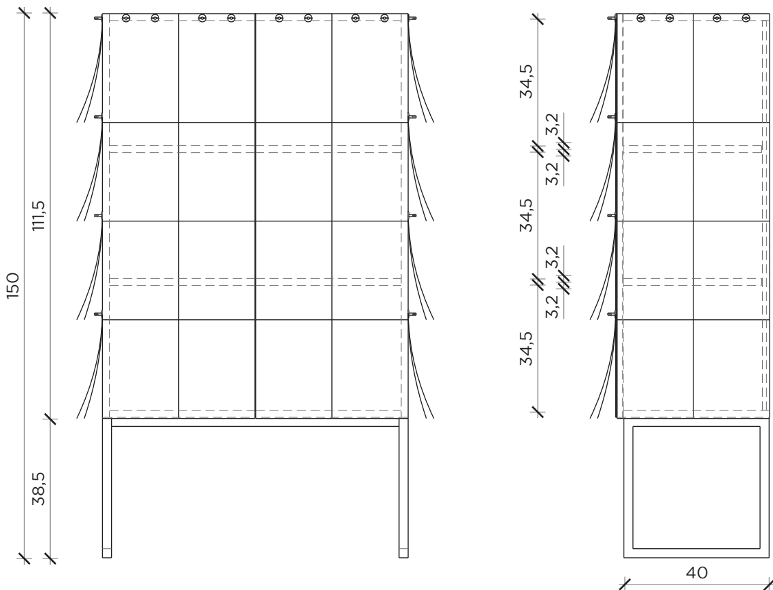
FRONTE | FRONT
