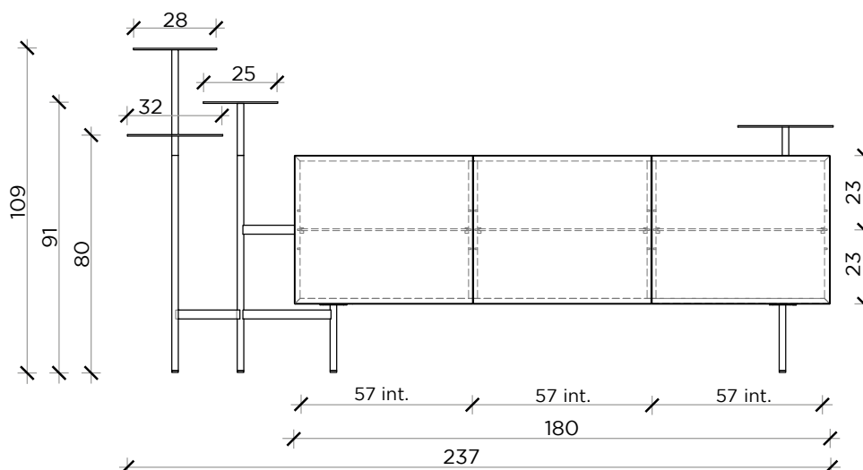
FRONTE | FRONT
