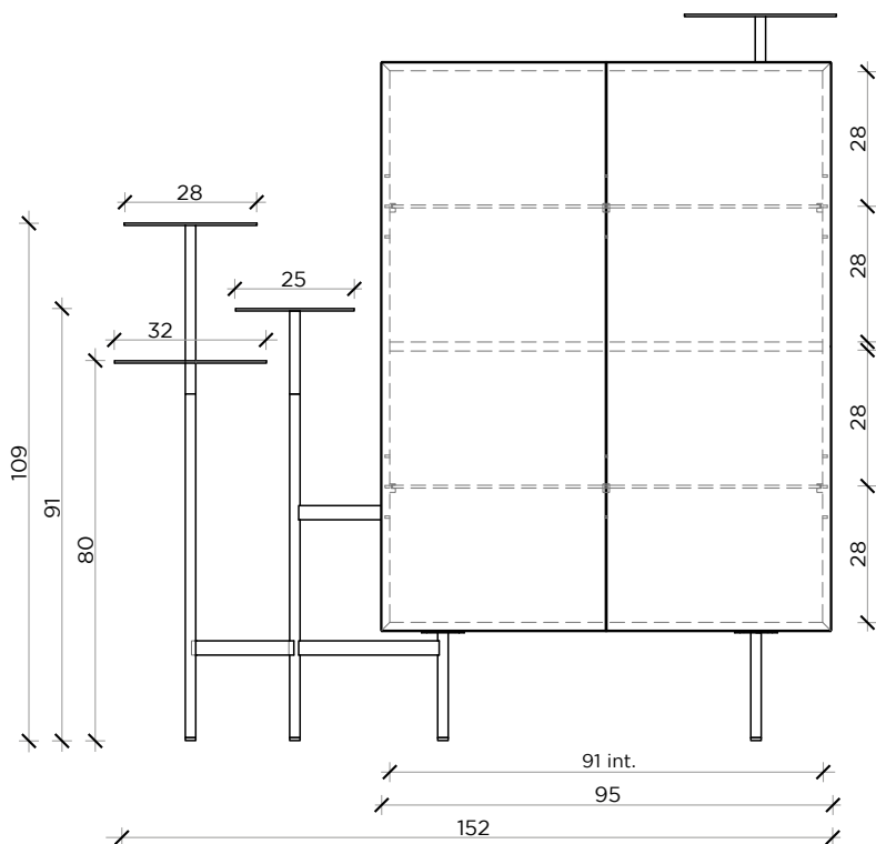
FRONTE | FRONT
