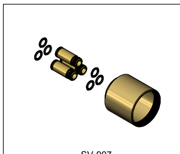
SV-907 Porta Cartucho p/ Monomando Cartridge Holder
