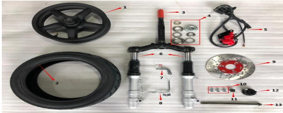
Figure C:front wheel,front shock,etc(图C:前轮、前减震等)
