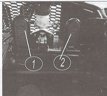
2. Accelerator Pedal
