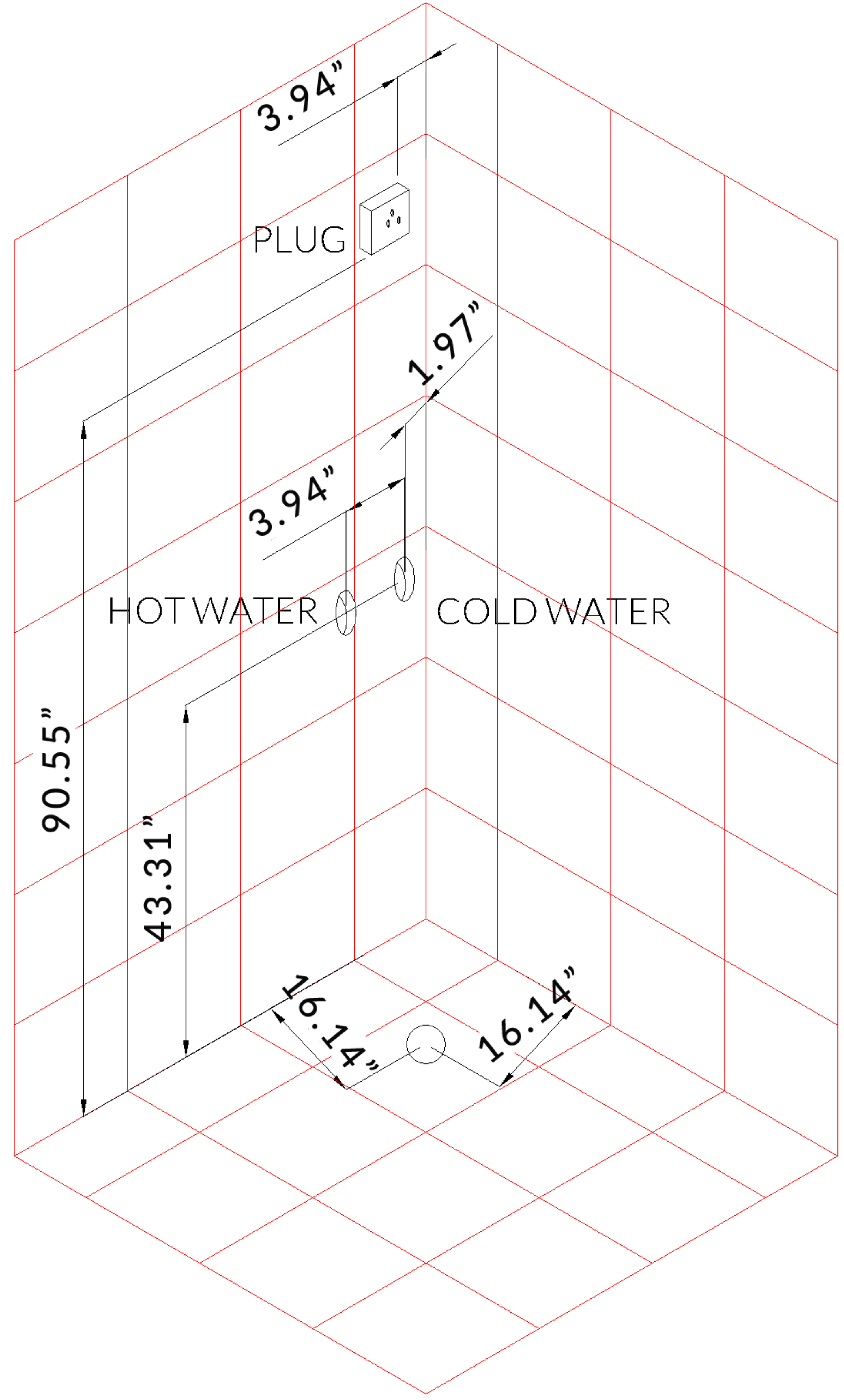
DZ960F8 INSTALLATION (LEFT) DIMENSIONS: 39" x 35" x 89"
