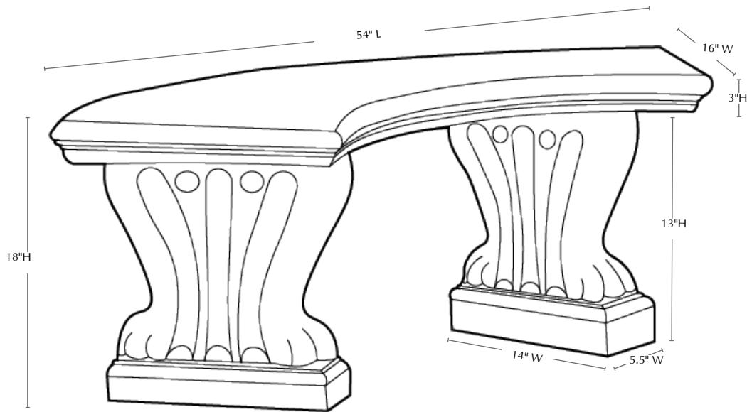
Isometric View
