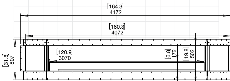
158RC.BX2 (LEFT & RIGHT DECORATIVE BOXES)
