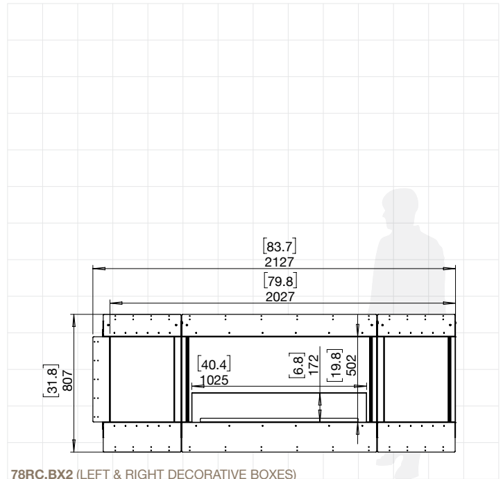
78RC.BX2 (LEFT & RIGHT DECORATIVE BOXES)
