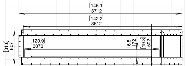
140RC.BXR (RIGHT DECORATIVE BOX)
