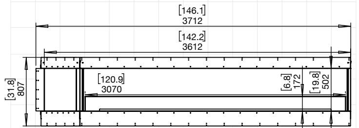
140RC.BXL (LEFT DECORATIVE BOX)
