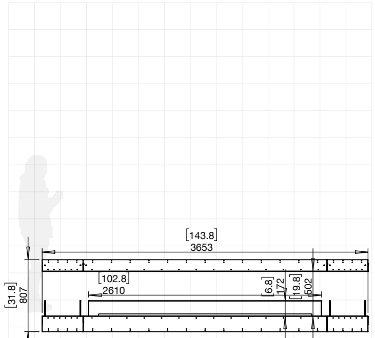
140IL.BX2 (LEFT & RIGHT DECORATIVE BOXES)
