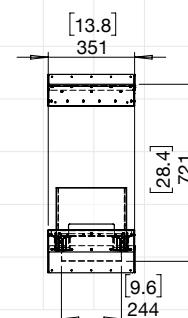
104IL.BX1 (LEFT DECORATIVE BOX)
