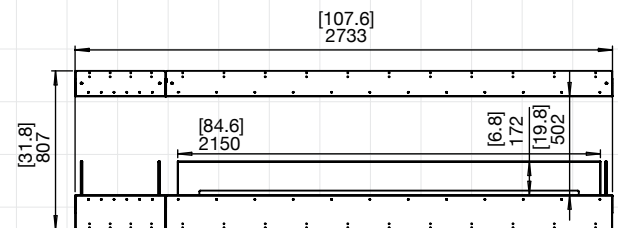
104IL.BX1 (LEFT DECORATIVE BOX)
