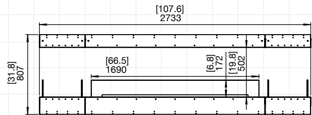
104IL.BX2 (LEFT & RIGHT DECORATIVE BOXES)
