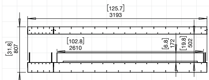
122IL.BX1 (LEFT DECORATIVE BOX)
