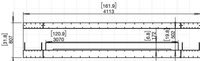
158IL.BX2 (LEFT & RIGHT DECORATIVE BOXES)
