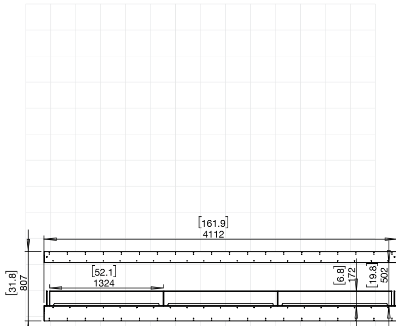
158IL (FLAME ONLY)
