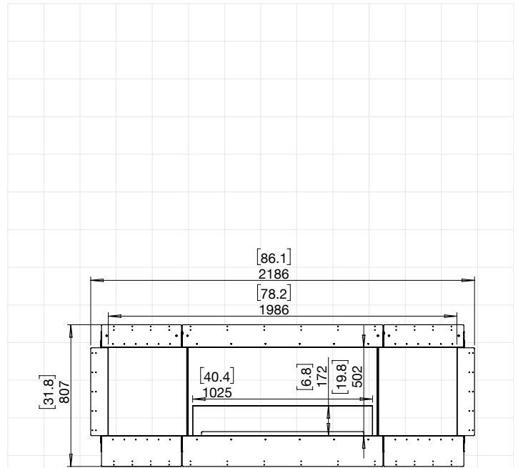
78DB.BX2 (LEFT & RIGHT DECORATIVE BOXES)
