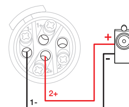
Bridge-Tied Load Wiring
