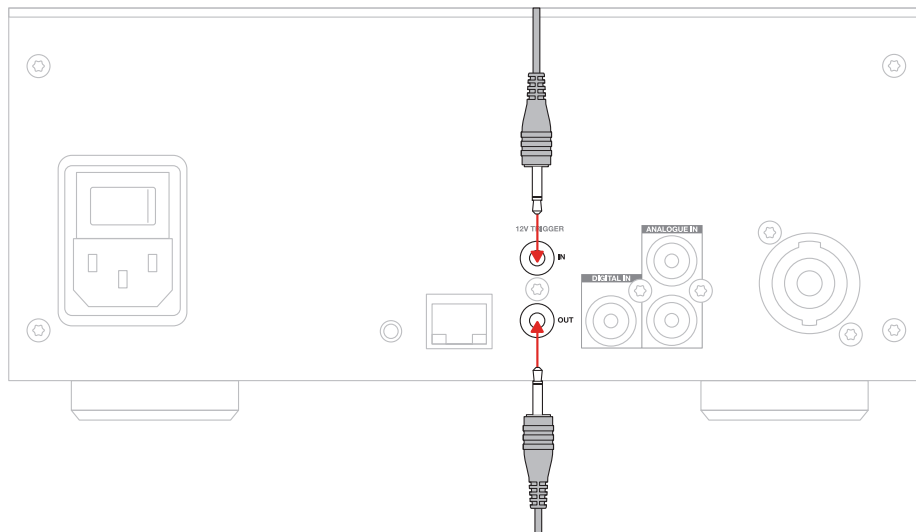
Diagram 12. 12V Trigger
