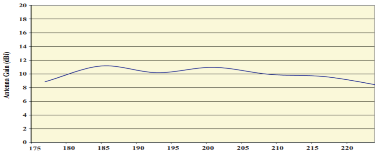
Antenna Gain (dBi) vs. Frequency (MHz)
