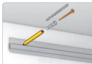
Mount the rails to the wall
