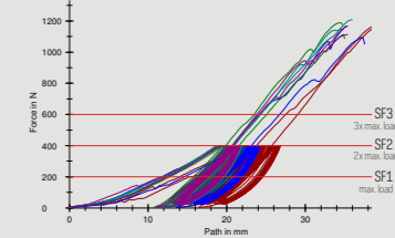
example of Micro Grip test results
