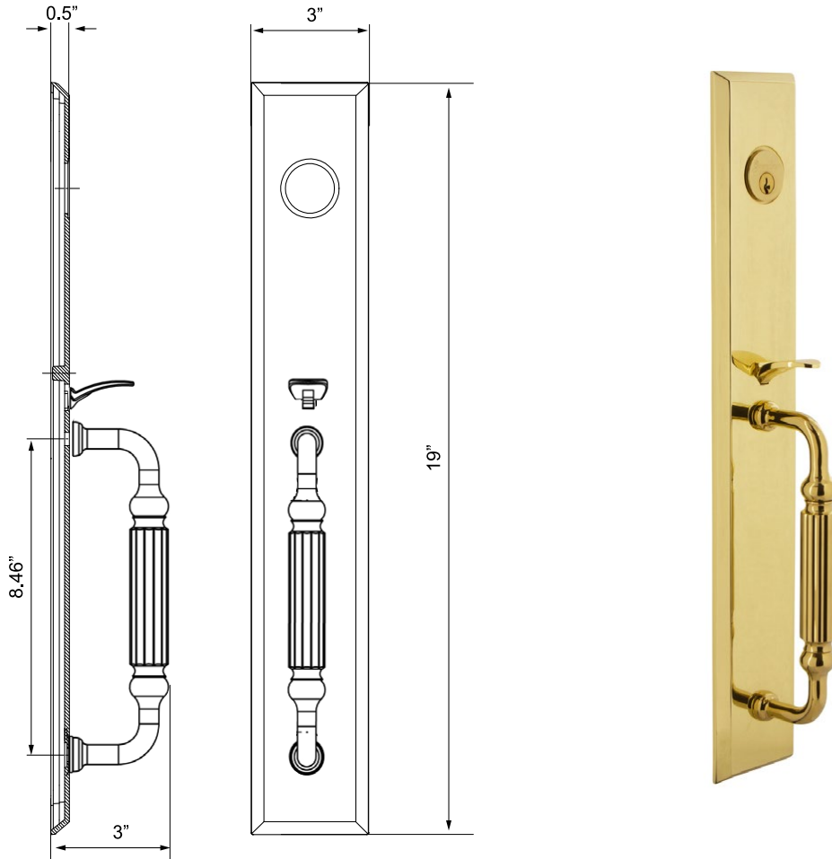
Fifth Avenue One-Piece Handleset with F-Grip in Lifetime Brass
