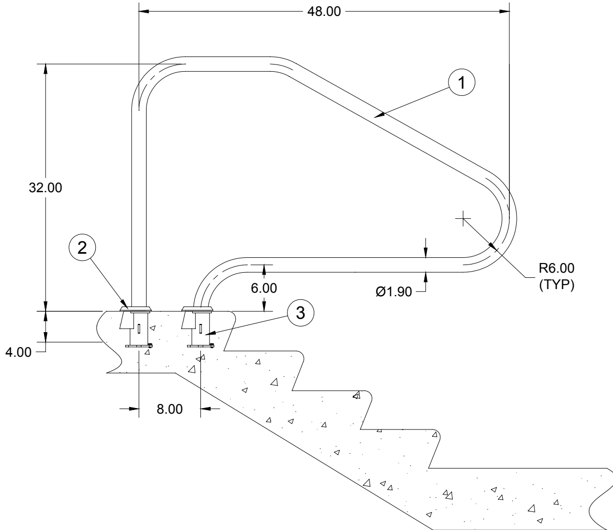
SIDE VIEW
