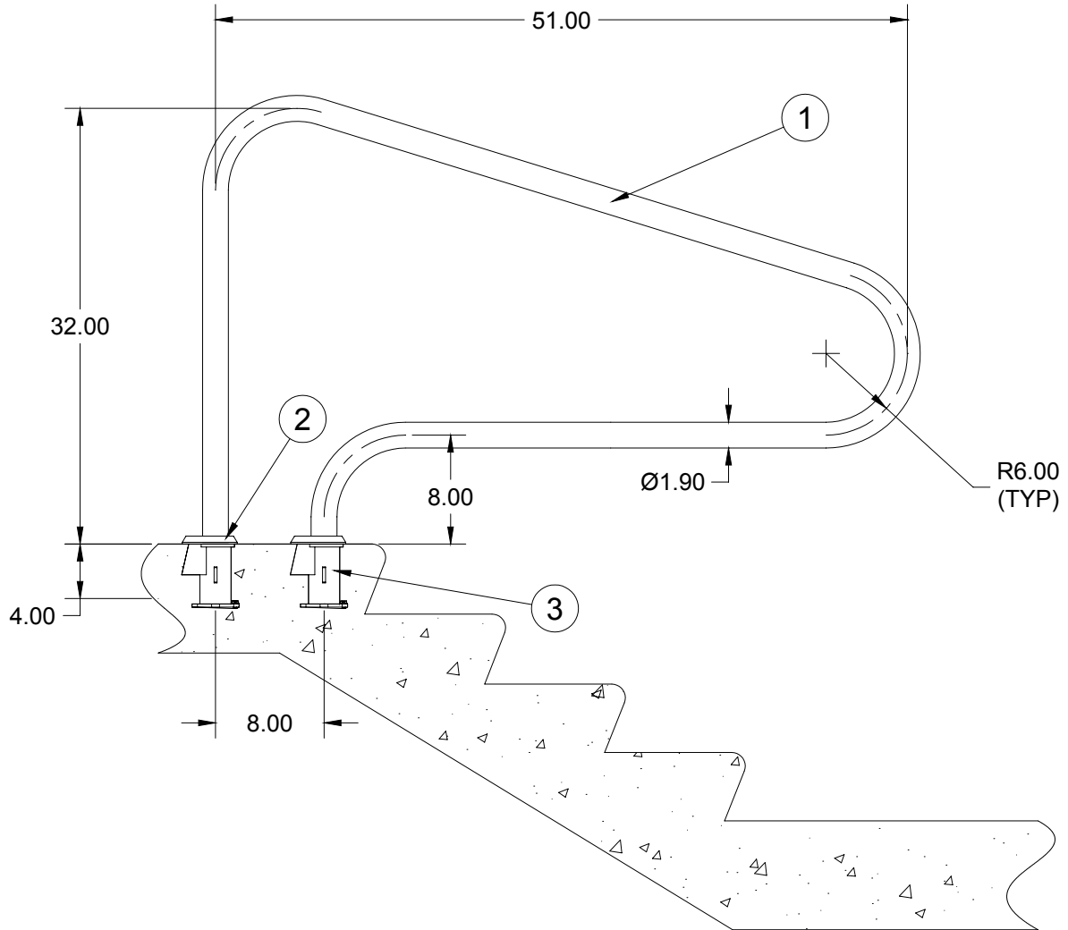
SIDE VIEW
