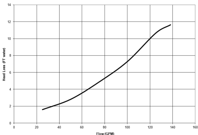
Head Loss Top Manifold
