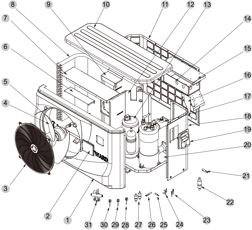
(1) Complete machine structure explosion diagram
