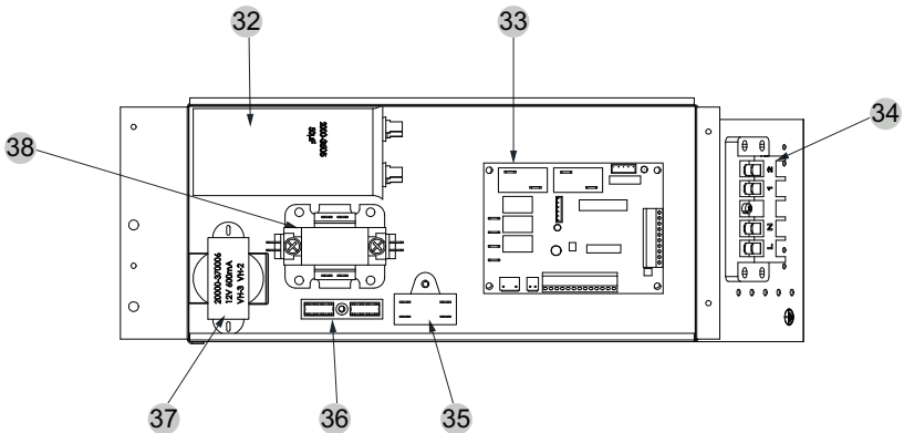
(2) Electrical control structure explosion diagram
