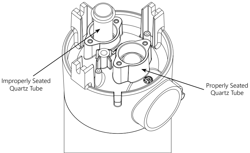
Figure 7: UV Quartz Tube Installation
