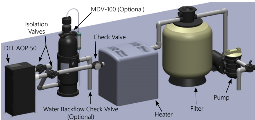
Figure 3: DEL AOP 50 Location in Pool Loop
