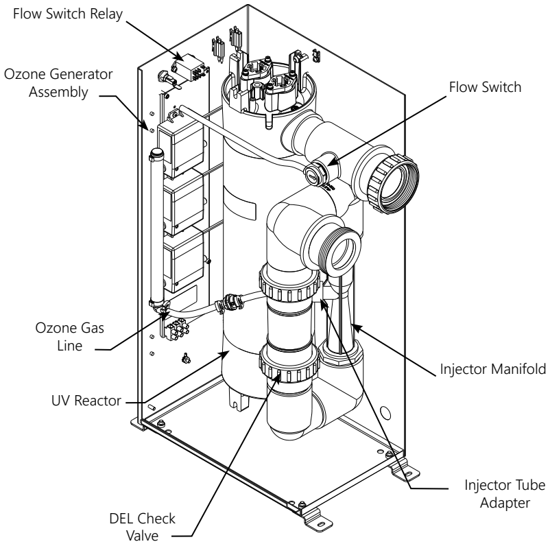
Figure 4: DEL AOP 50 Electro-Mechanical Overview
