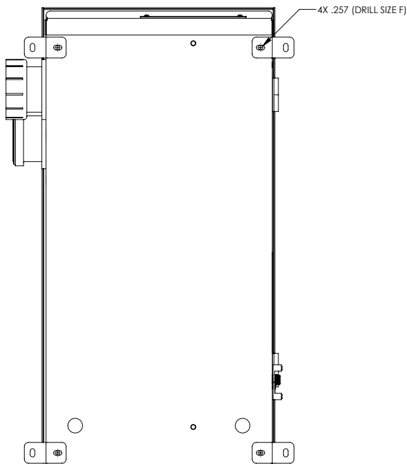
Figure 2: Wall Mounting Hole Pattern
