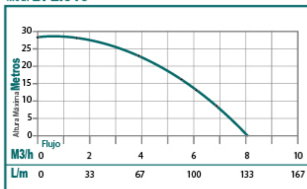
Mod. BP2.510
