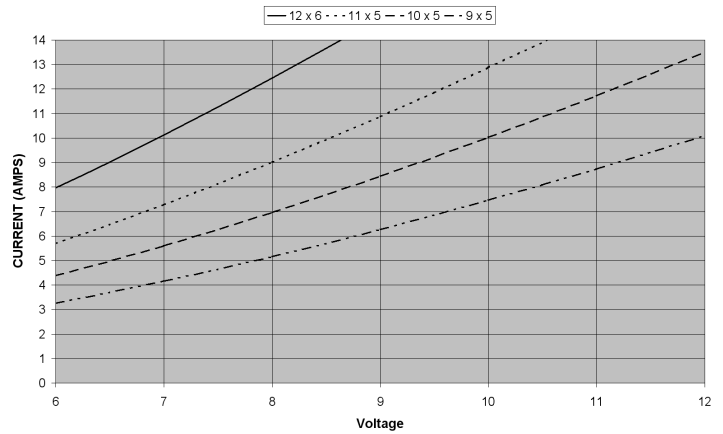
HC2812-0850 Current vs. Voltage with propeller
