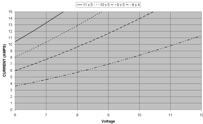
HC2812-1080 Current vs. Voltage with propeller
