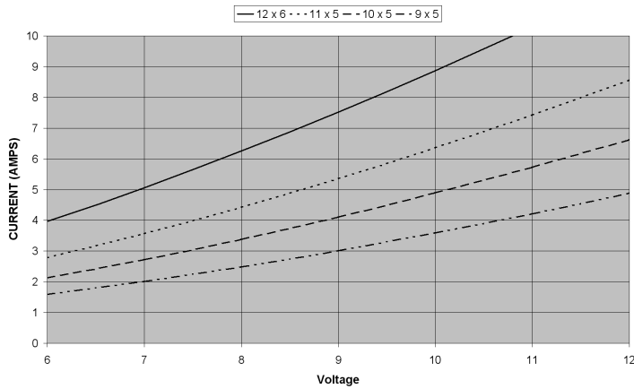
HC2812-0650 Current vs. Voltage with propeller
