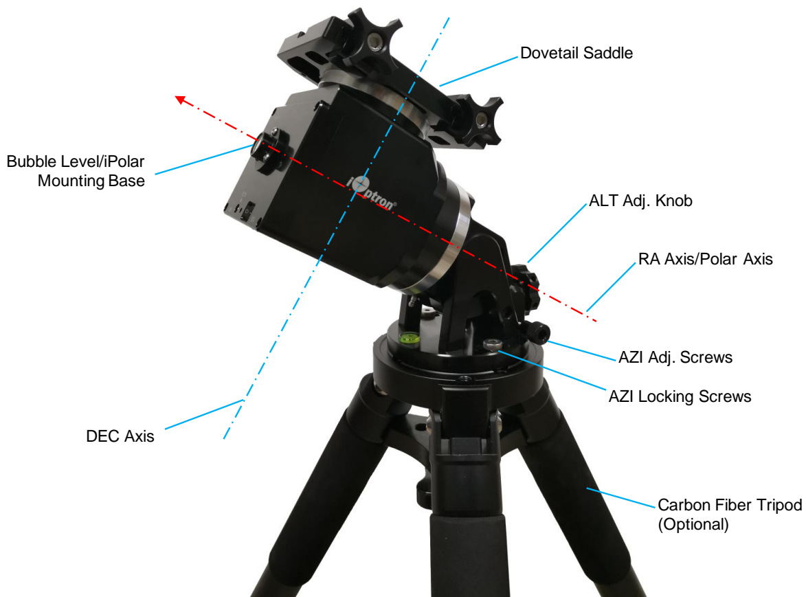
Figure 1. HAE mount assembly
