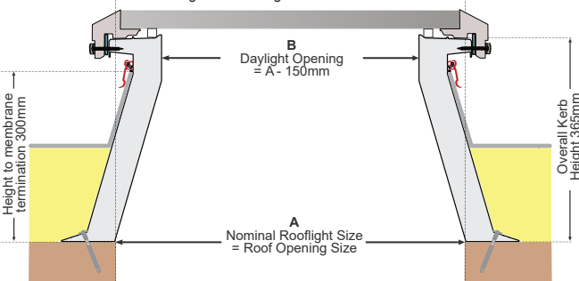
Figure 4: Rooflight with 300mm PVC kerb
