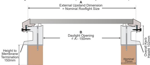
Figure 2: opening / ventilated rooflight on builders upstand
