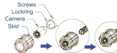
Figure 13. 72 Roller skid
