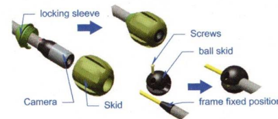
Figure 15. 78 Roller skid
