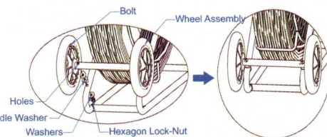
Figure 20. Install the wheel assembly
