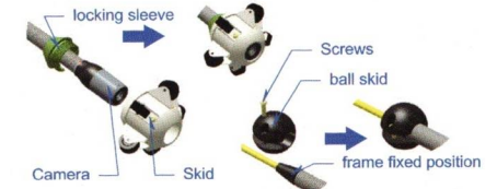
Figure 16. 134 Roller skid
