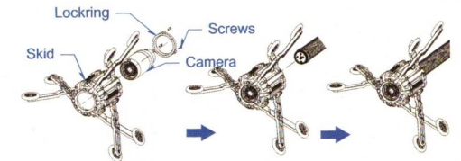
Figure 14. 120 Roller skid
