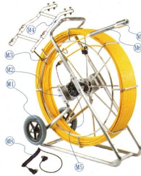
Figure 9. Frame assembly
