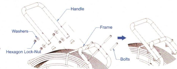
Figure 17. Install handle
