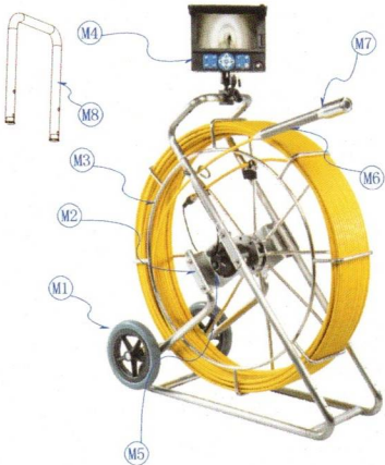
Figure 7. Frame assembly
