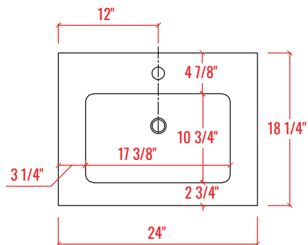
ELEVATION VIEW
