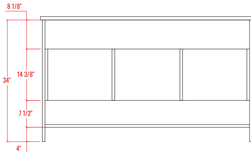
BACK VIEW
