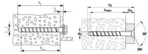
ULTRACUT FBS II 8 - 12 A4 - SK - countersunk head
