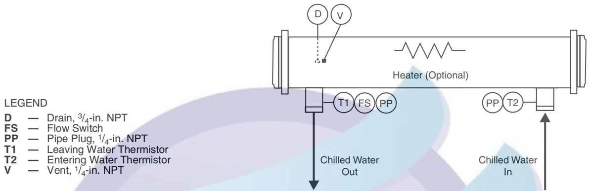
TYPICAL PIPING DIAGRAM FOR 30RB UNITS WITHOUT HYDRONIC PACKAGE
