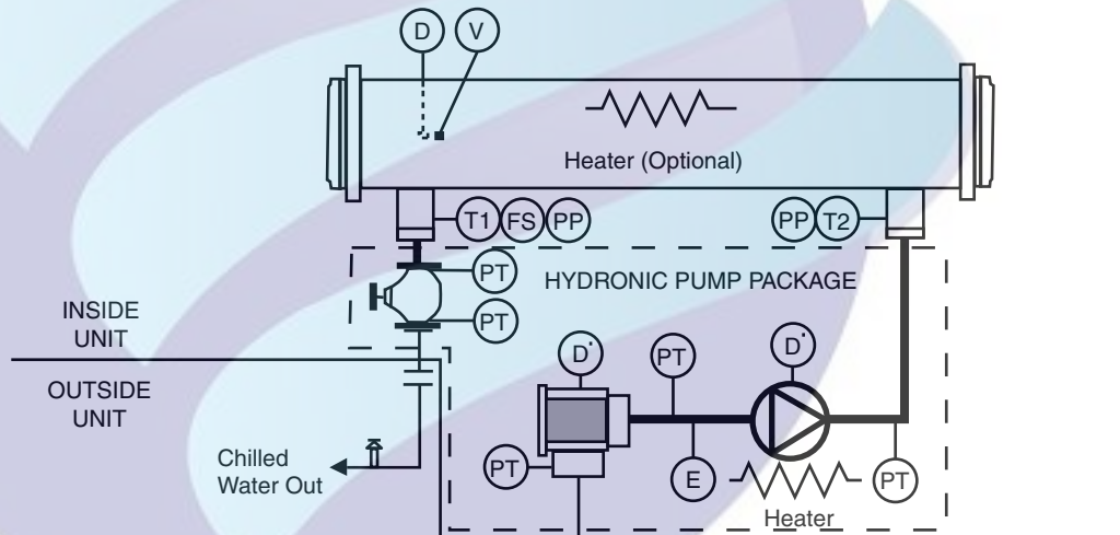
TYPICAL PIPING DIAGRAM FOR 30RB UNITS WITH HYDRONIC PACKAGE — SINGLE PUMP
