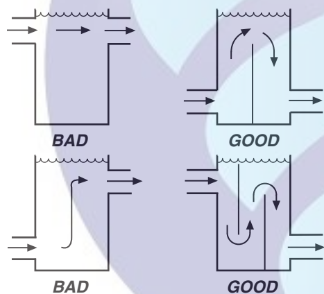
Fig. 35 — Tank Baffling
