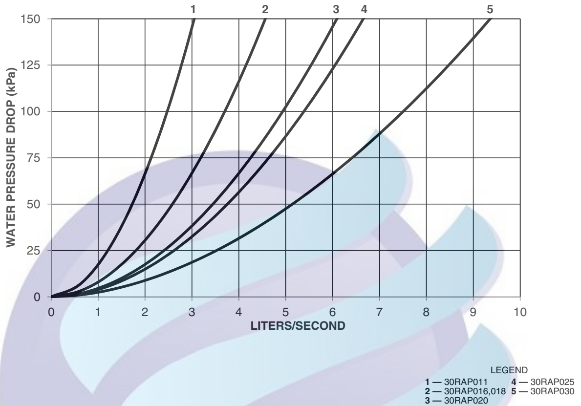
Fig. 31 — Heat Exchanger Pressure Drop (Water Only) — 30RAP011-030 (SI)
