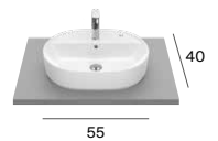
The Gap A3270Y0000
