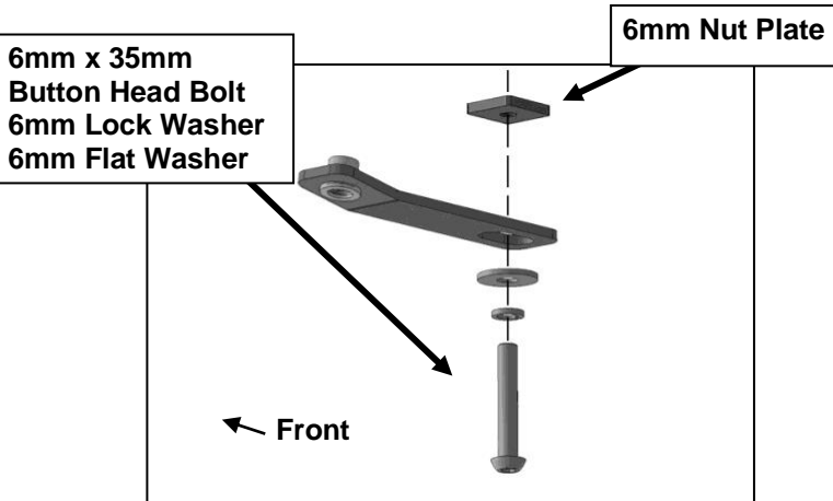
(Fig 9) Attach (4) Splash Guard Support Brackets to the bottom of the center splash guard
