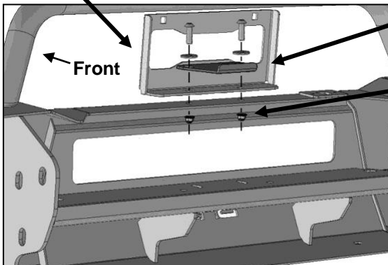
(Fig 11) Models without winch, attach Grille Support Bracket and License Plate Bracket (if required)
