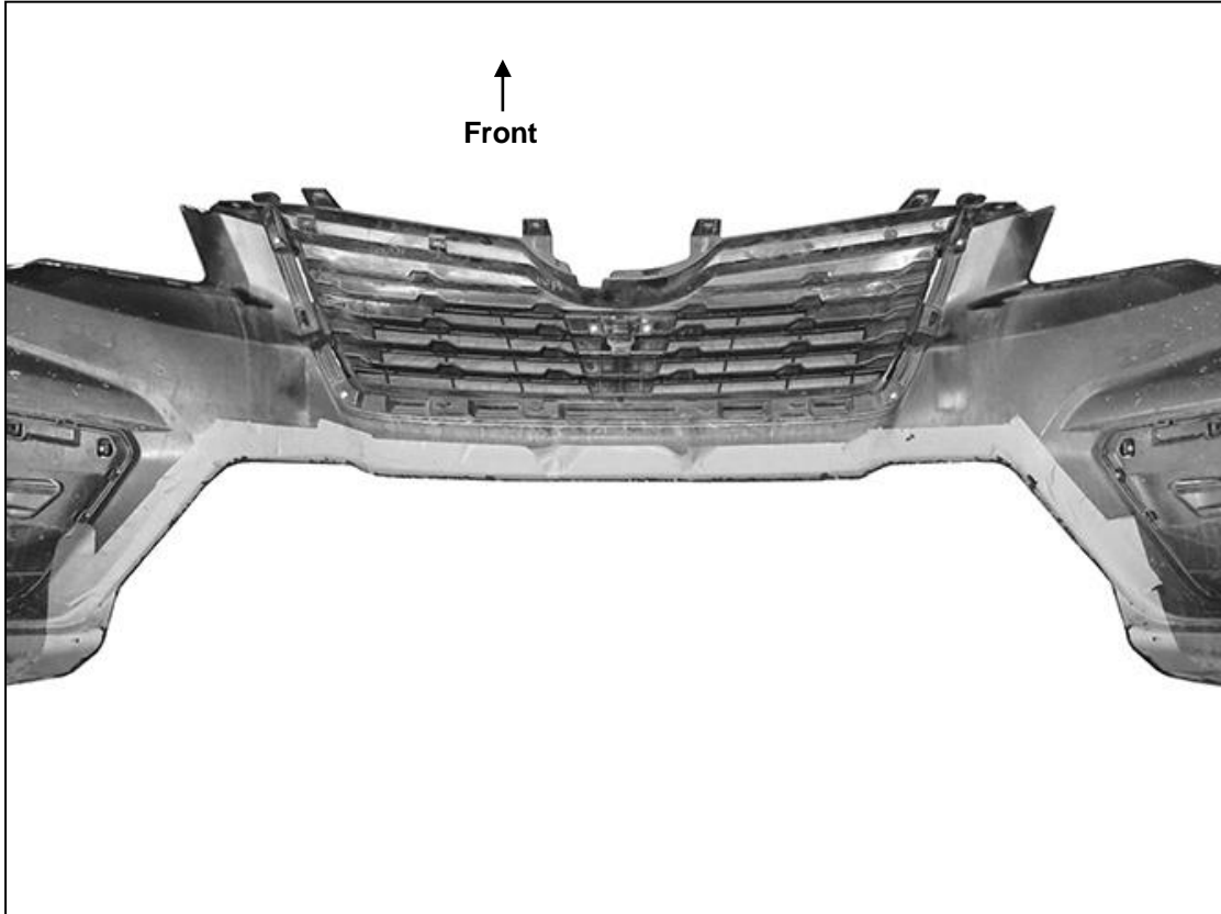
(Fig 26) After checking the fit of the bumper cover to the Hiline Bumper, remove the tape and apply the included Edge Trim (cut to fit), and reinstall bumper cover
