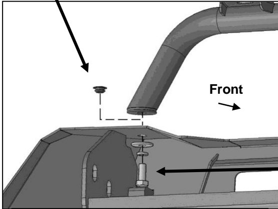
(Fig 10) Remove rubber plug to attach Bull Nose Hoop to top of Bumper
