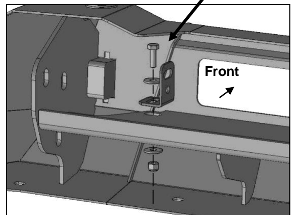
(Fig 12) Models without winch, attach "L" Brackets to mounting holes in tray. Attach LED bar style light (not included) to "L" Brackets
