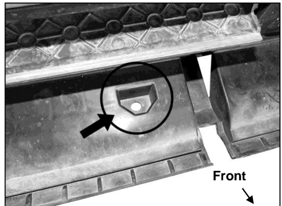
(Fig 8) Insert (1) 6mm Nut Plate into each of the (4) pockets in the center splash guard (see Fig 9)
