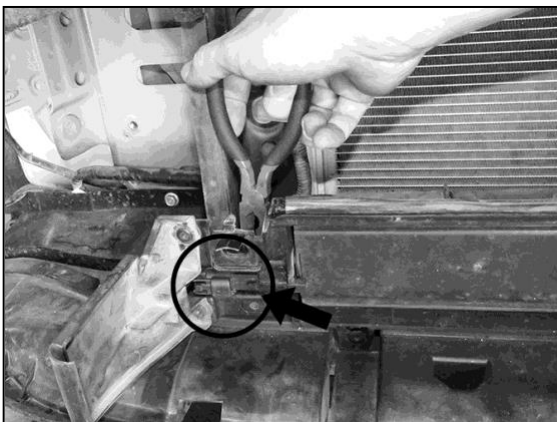
(Fig 7) Use needle nose pliers to reach in and release the tab on the sensor located on the passenger/right side
