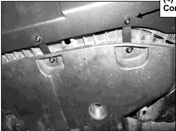
(Fig 23) Attach Splash Guard Support Brackets to back of Bumper (also see Fig 8)
