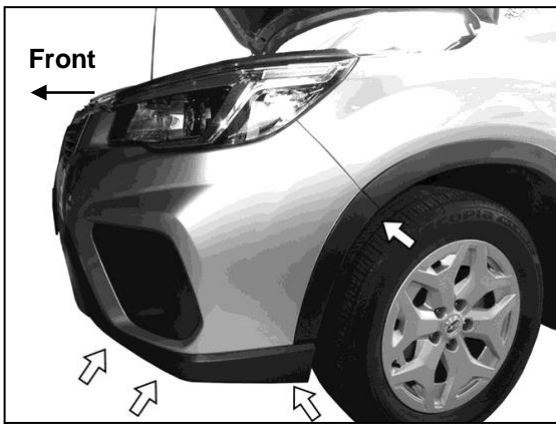
(Fig 1) Remove clips attaching ends and bottom of plastic bumper cover (arrows)
