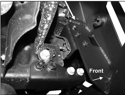
(Fig 18) Attach Bumper to Frame Brackets
