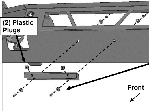
(Fig 14) Attach License Plate Bracket to Bumper
