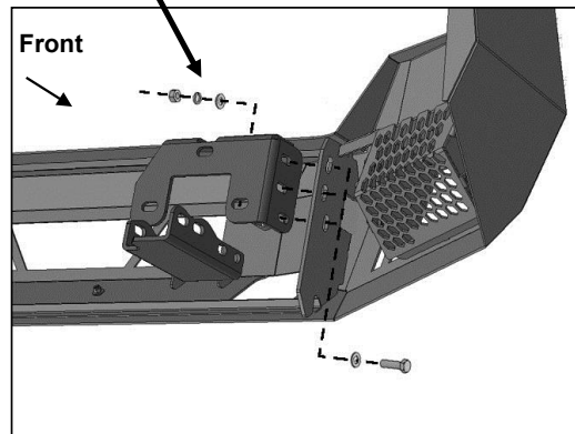
(Fig 17) Attach the Bumper to Frame Bracket
