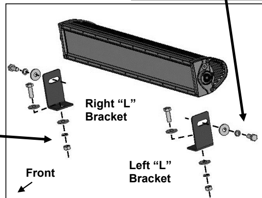
(Fig 15) Typical center light installation
