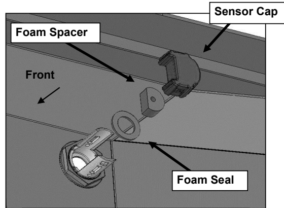
(Fig 13) Slide sensor into sleeve, insert Foam Spacer and snap on Cap to lock sensor in sensor mount
