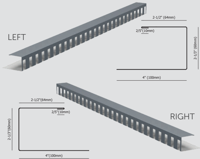
VALLEY FLASHING FOR SUPRE/ULTRA/COMO L=4 ft (1220 mm)
