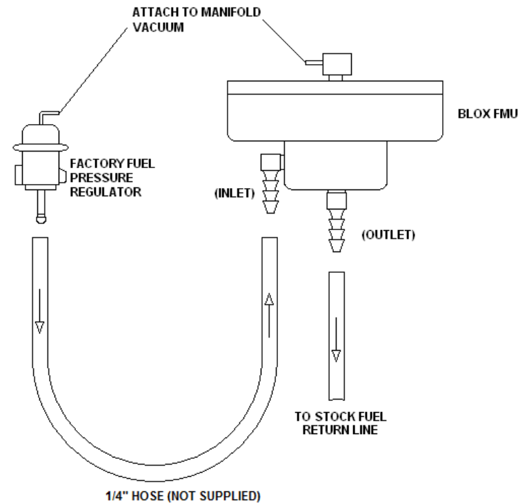
BLOX RACING FMU ASSEMBLY DIAGRAM
