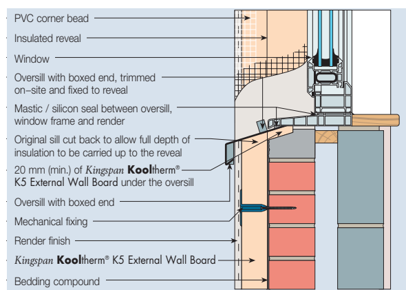
Figure 9 – Oversill Extension Detail (Refurbishment)
