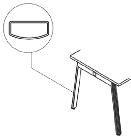
Yan M - powder coated steel, profile 60 x 30 mm Worktop – MFC 28 mm, ABS edge
