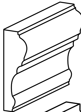
Ogee Cap OG-CAP1 Group C Corners: IP, LP, RP 4 5/8" H x 6" L x 1 1/2" D
