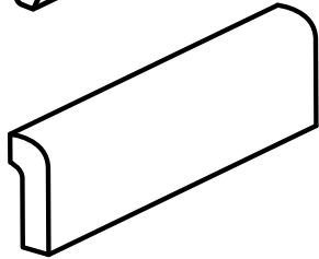
Radius Bullnose ST-R261 Group B Corners: DA, UA, IC, OC 1 7/8" H x 6" L x 7/8" D
