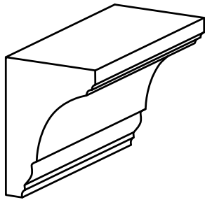
Ceiling Cove C ST-CCCI Group C Corners: IP, RP, LP 3 3/4" H x 6" L x 2 1/4" D
