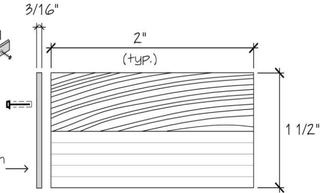
CRITICAL DIMENSIONS (Do not scale)
