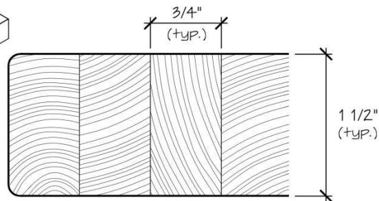
CRITICAL DIMENSIONS (Do not scale)
