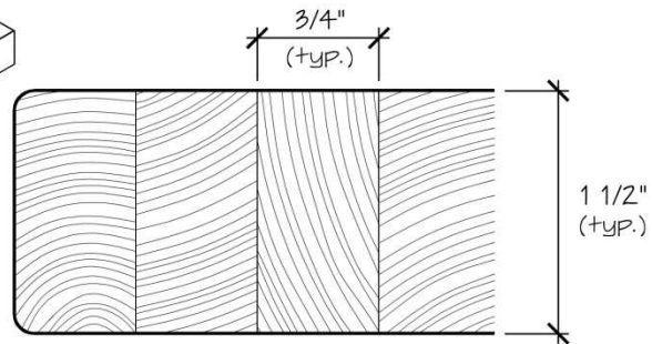
CRITICAL DIMENSIONS (Do not scale)
