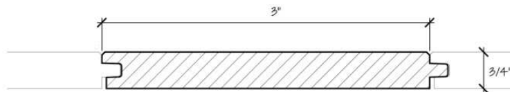
CRITICAL DIMENSIONS (Do not scale)
