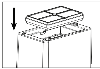
d. Insert Combination Filter into the unit with the HEPA portion facing into the unit. Consult the arrow on the filter for correct installation direction.
