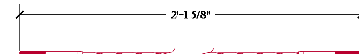
Ø1/8" SHORT CABLE W/ SWAGE STUDS : QTY- 5
