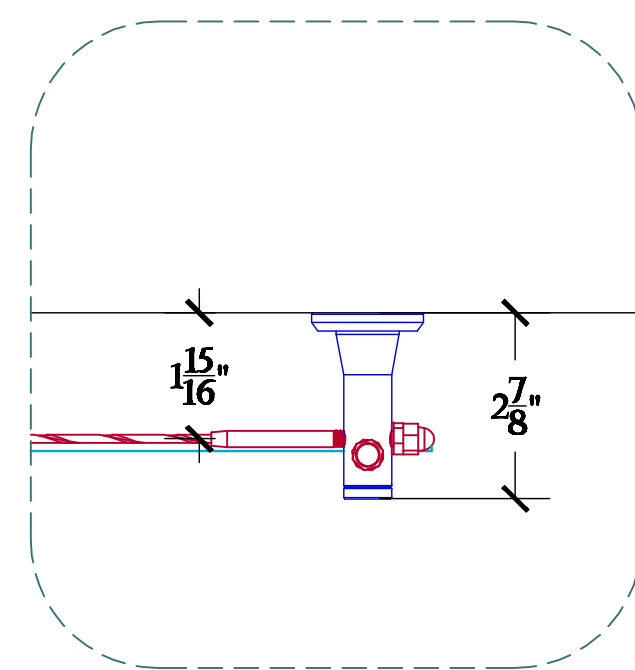
TOP VIEW DETAIL.
