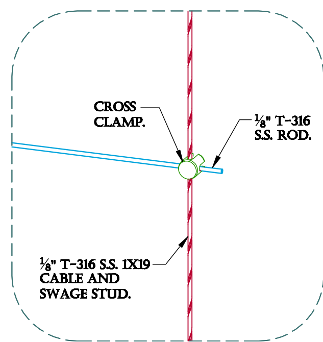
MOUNTING DETAIL 3.
