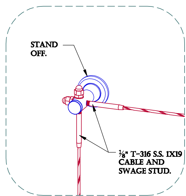
MOUNTING DETAIL 1.
