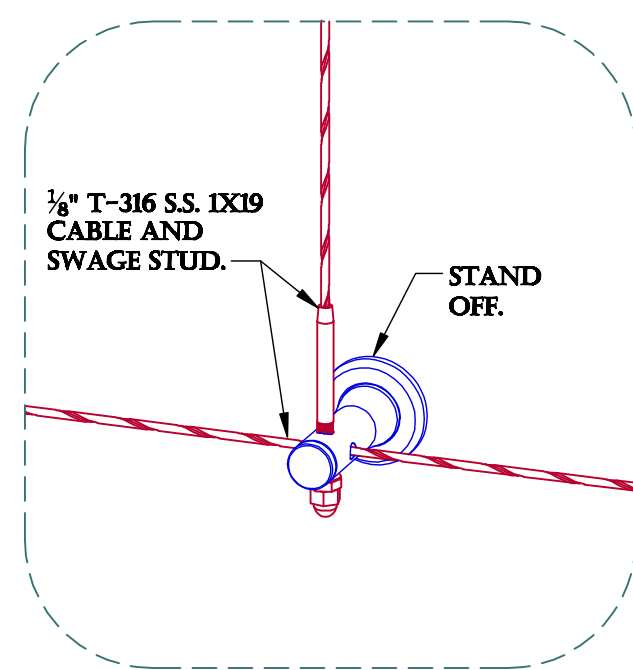
MOUNTING DETAIL 2.
