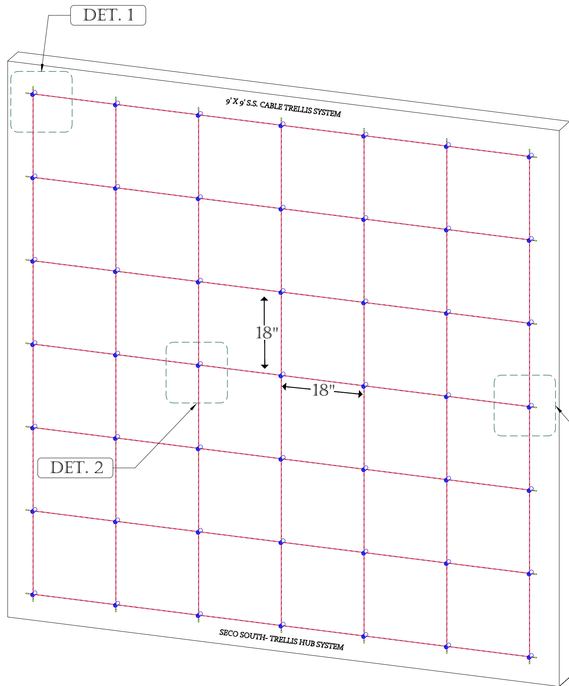
9' X 9' TRELLIS, 18" GRID.
