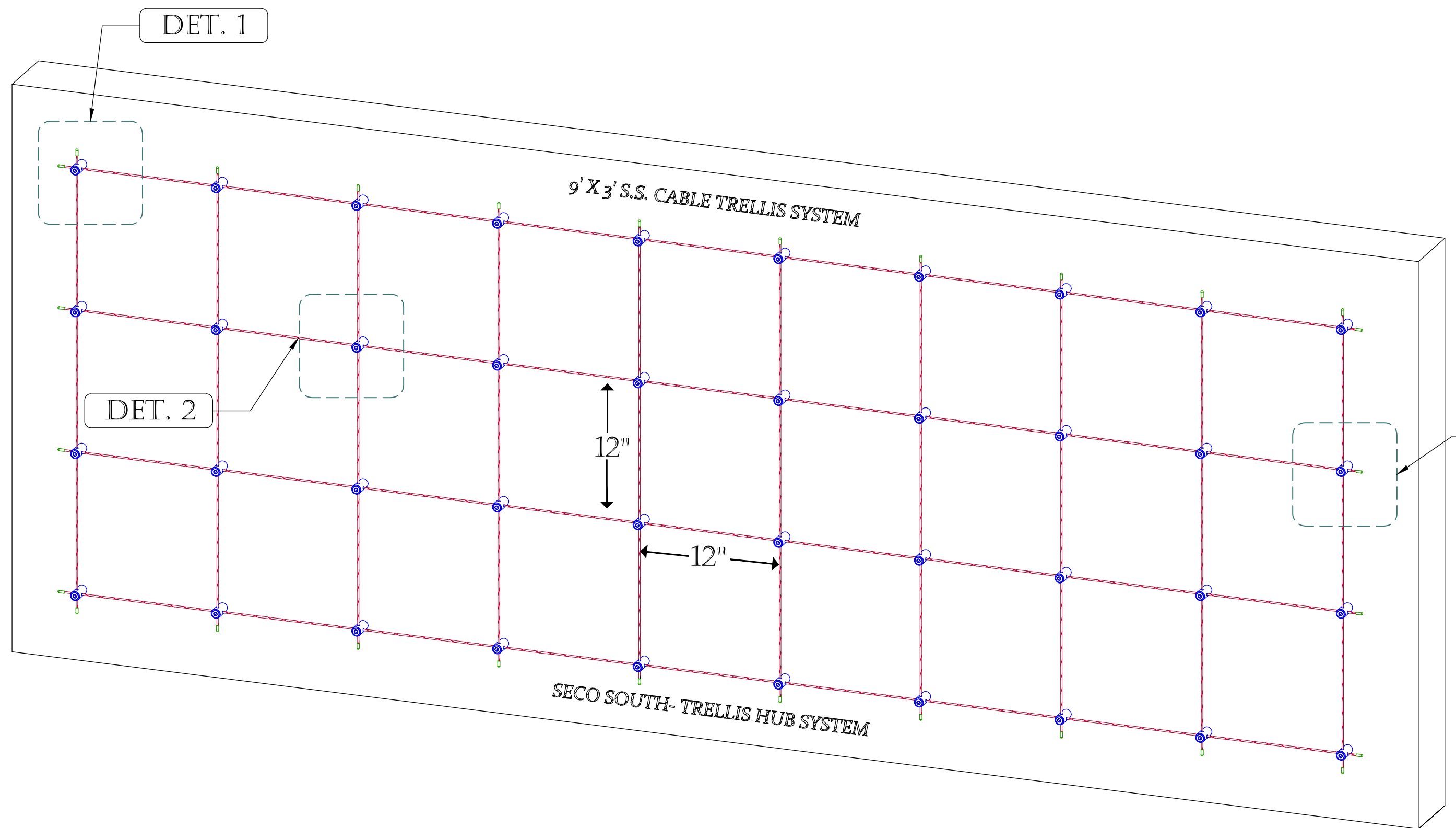
9' X 3' TRELLIS, 12" GRID. SCALE: 1 1/2" = 1'
