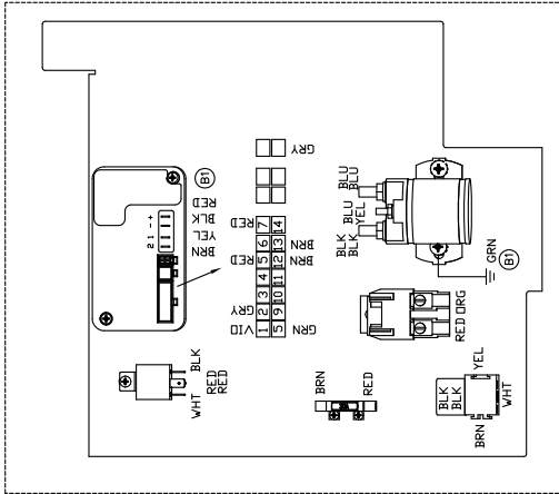
ELECTRICAL PANEL
